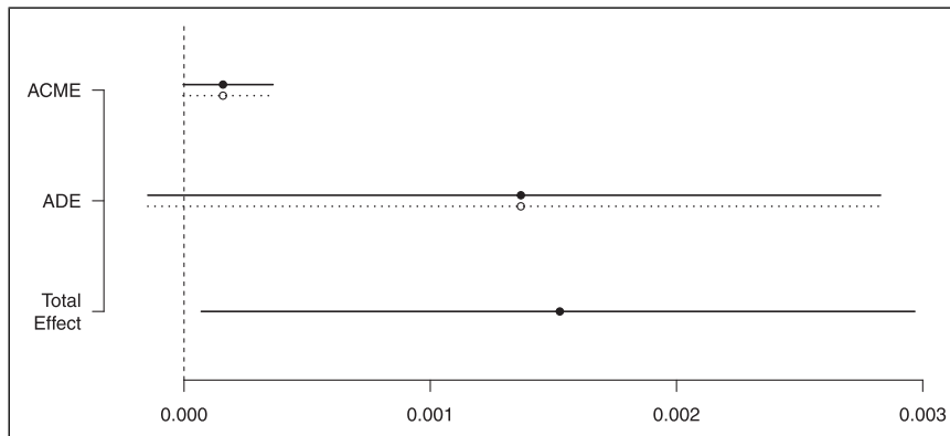
Figure A4. Mediation analysis.
