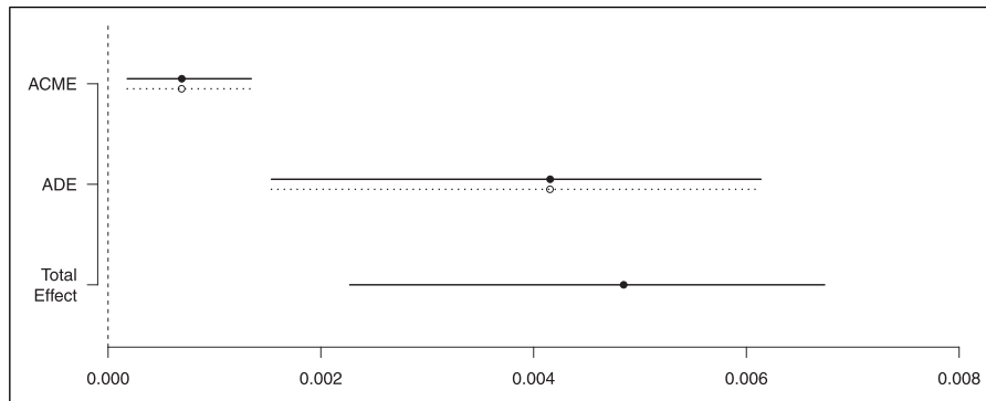
Figure A3. Mediation analysis.
